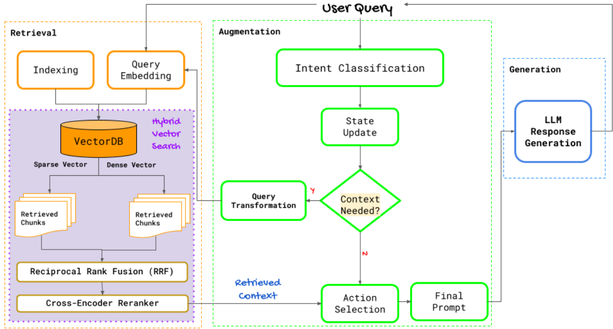
Figure 1: Overview of our Hybrid RAG architecture for a C-TRS. The pipeline operates in a multi-turn setting, where user utterances are parsed to extract context and intent. Based on the dialogue state, relevant city-level chunks are retrieved from a hybrid semantic index (combining dense and sparse retrieval), optionally reranked, and used to augment the prompt for the LLM. The generation module produces grounded, context-aware responses for recommending European cities.
